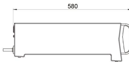
Supply unit tabletop device
