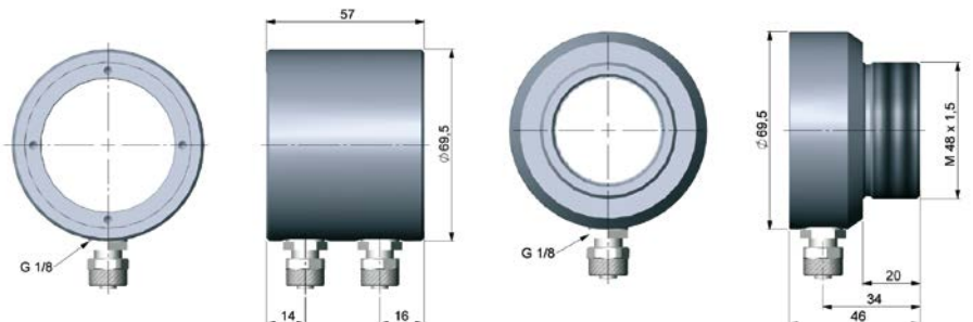
TM-W-CTL Water cooled housing
