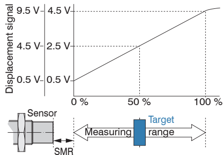
Fig. 4 Start of measuring range (SMR), the smallest distance between sensor face and measuring object
