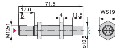
Fig. 2 DT3001-SA, dimensions in mm (not to scale)
