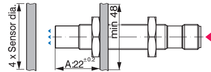
Fig. 5 Assembly, dimensions in mm (not to scale)
