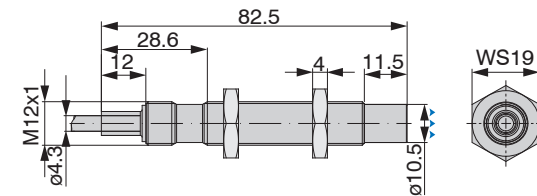
Fig. 3 DT3001-Cx, dimensions in mm (not to scale)
